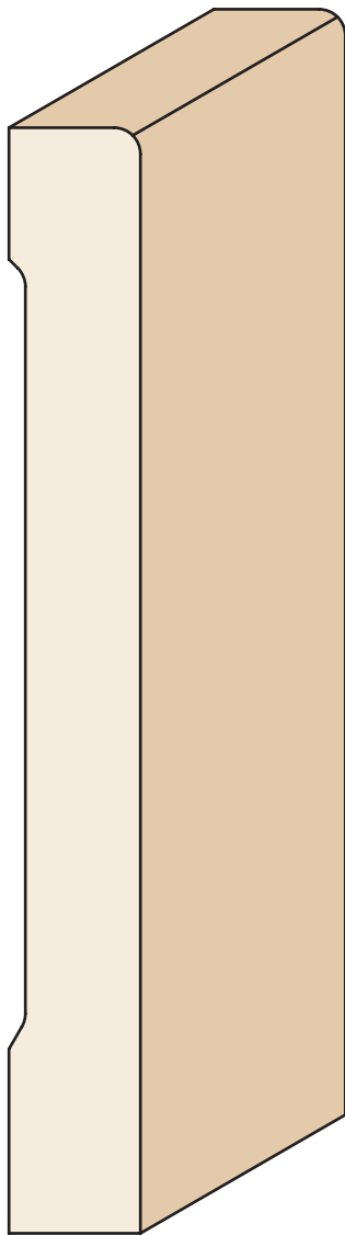
20168-1R18-B \frac{5}{8} " x 5\frac{1}{4} "
