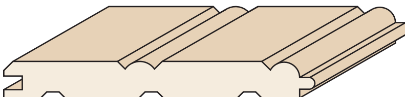
1296-TVG-BD \frac{3}{8} " x 3" (face)
