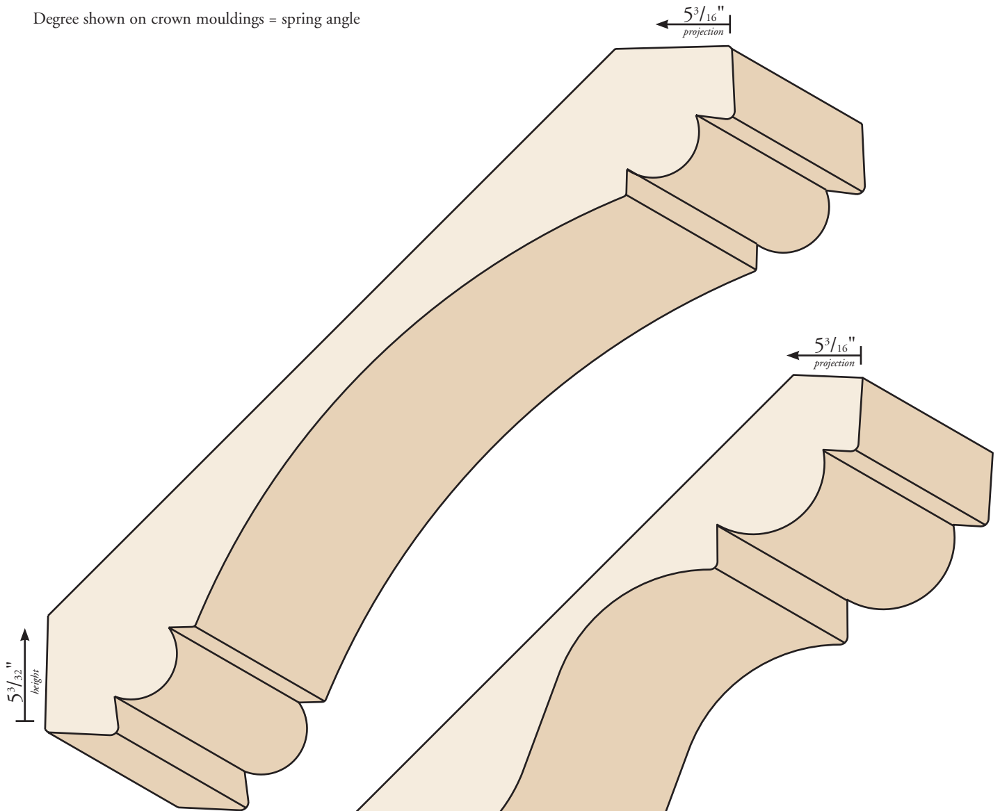
25M232-C-CR 25mm x 7\frac{1}{4} " (43.5°)
