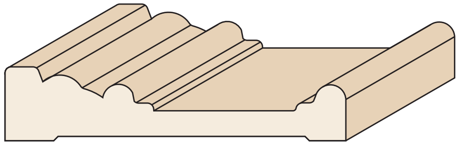
24112-CA 3/4" x 3 1/2"
