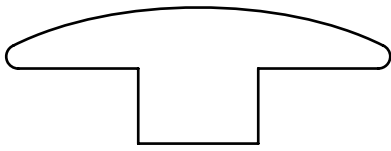
2364-FUS-T \frac{23}{32} " x 2" for \frac{3}{4} " floor
