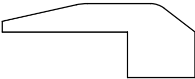
2668-S-THR \frac{13}{16} " x 2\frac{1}{8} "
