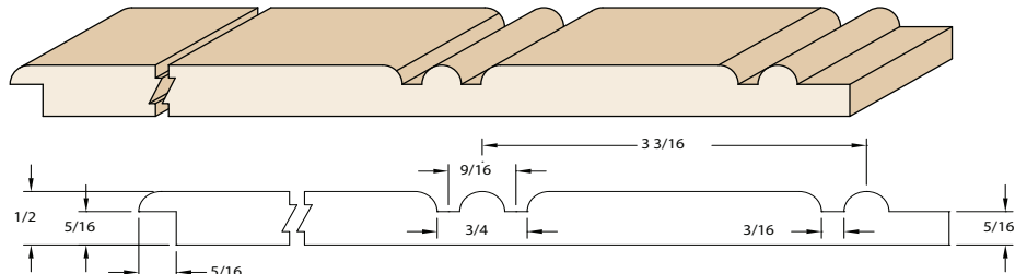
1/2" x 4' x 8' beaded, approx. 3-1/4" OC
