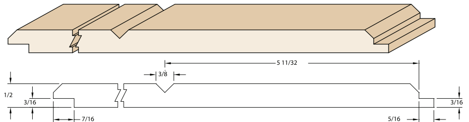
1/2" x 4' x 8' v-grooved, approx. 5-1/2" OC
